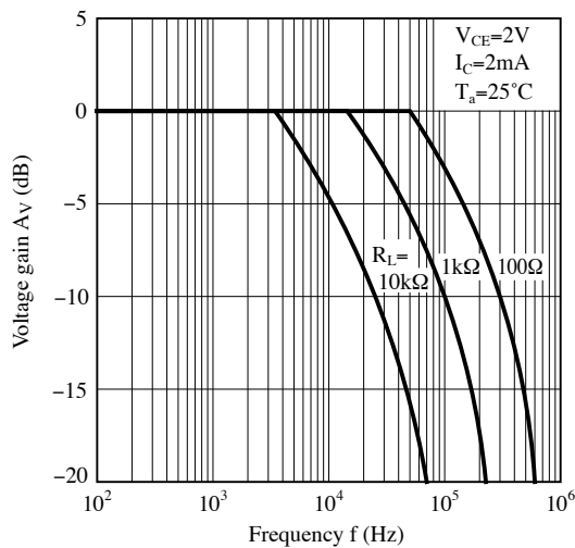
Fig.11 Frequency Response
