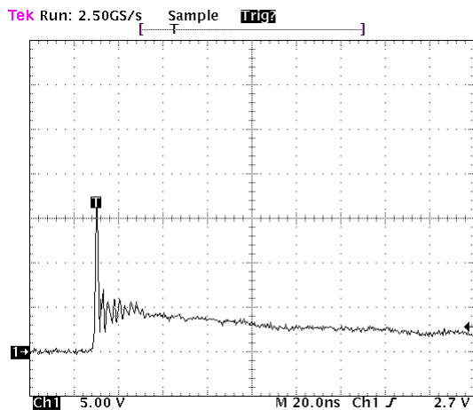
ESD Response (4kV Contact per IEC 61000-4-2)
