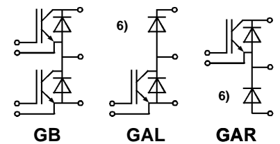
SEMITRANS 3
