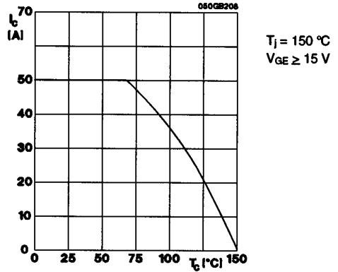
Fig. 8 Rated current vs. temperature I_{\text{C}} = f(T_{\text{C}})
