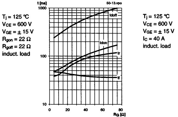
Fig. 16 Typ. switching times vs. gate resistor R g
