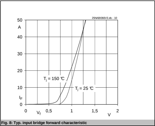
Fig. 8: Typ. input bridge forward characteristic
