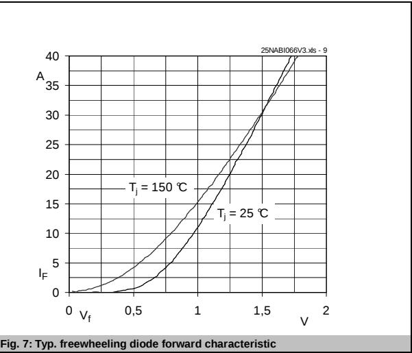
Fig. 7: Typ. freewheeling diode forward characteristic
