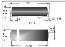
Surface mount diode
