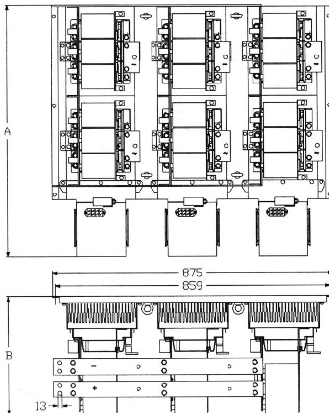
2.Application example using SKiIPs and heatsink P 16 to give an IGBT inverter
