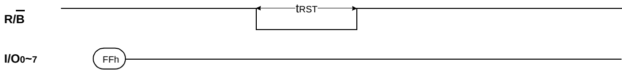
Figure 23. RESET Operation
