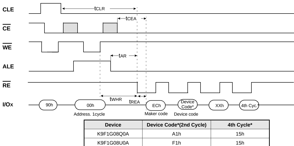
Figure 14. Read ID Operation
