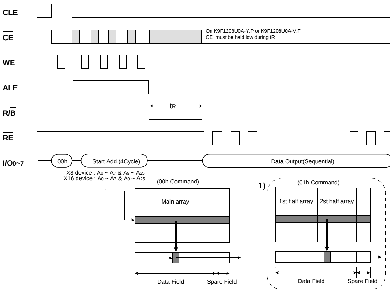
Figure 7. Read1 Operation
