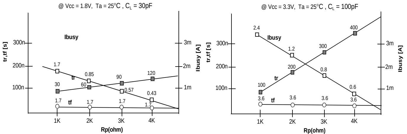
Fig 23 R_p vs t_r , t_f & R_p vs i_{\text{busy}}
