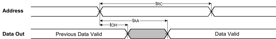
TIMING WAVEFORM OF READ CYCLE(1) ( \overline{CS}=\overline{OE}=V_{IL}, \overline{WE}=V_{IH} )
