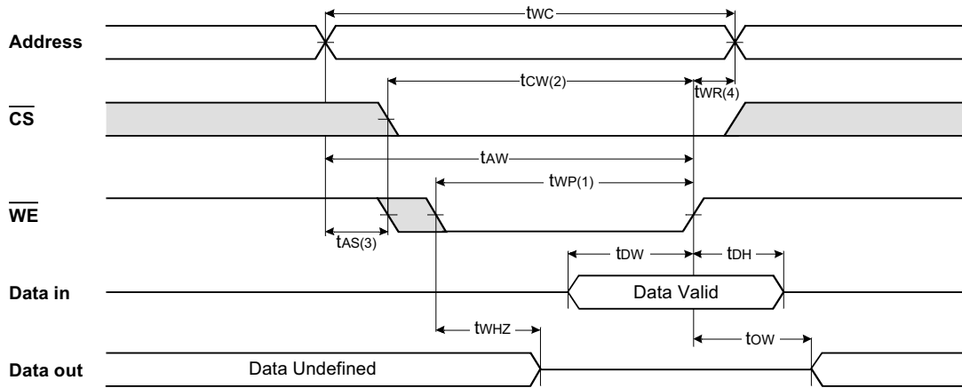
TIMING WAVEFORM OF WRITE CYCLE(2) ( \overline{CS} Controlled)
