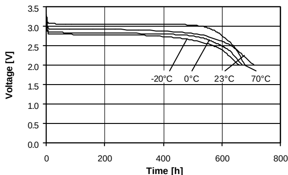
Temperature performance Load 16.2kW
