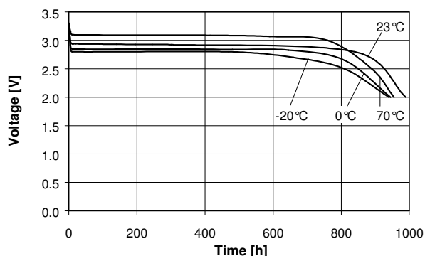
Temperature performance Load 12kΩ
