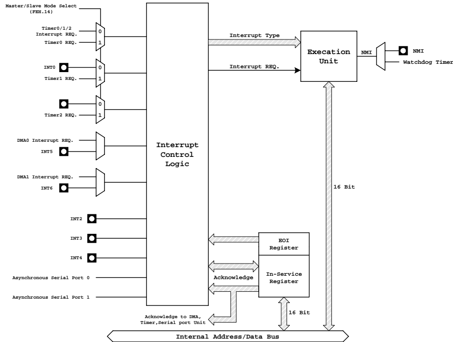
Interrupt Control Unit Block Diagram
