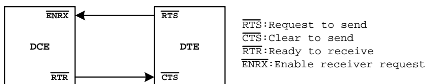
DCE/DTE Protocol Connection
