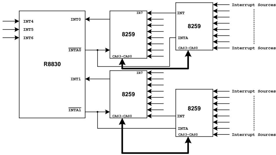
Cascade Mode Connection
