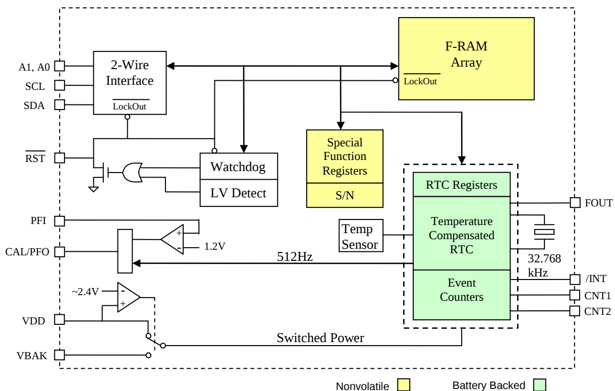
Figure 1. Block Diagram
