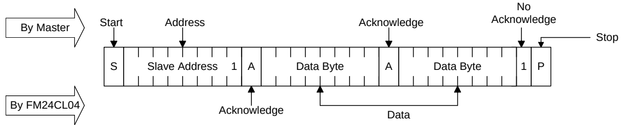
Figure 8. Sequential Read
