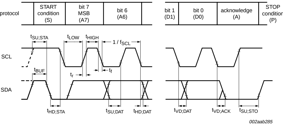
Fig 15. I 2 C-bus timing diagram
