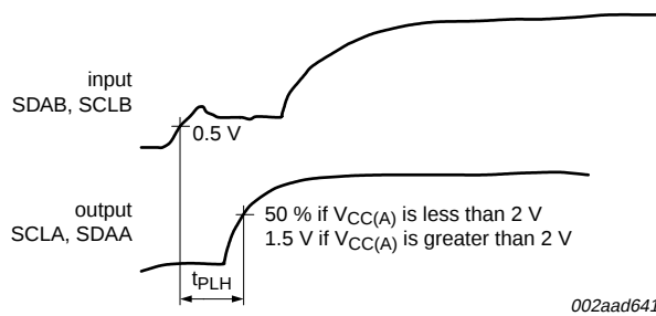
Fig 10. Propagation delay and transition times; port B to port A
