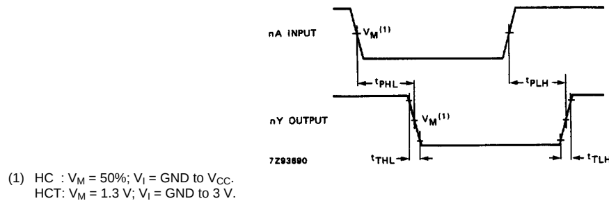
Fig.6 Waveforms showing the input (nA) to output (nY) propagation delays and the output transition times.
