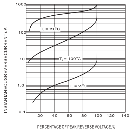
Fig.4-TYPICAL REVERSE CHARACTERISTIC
