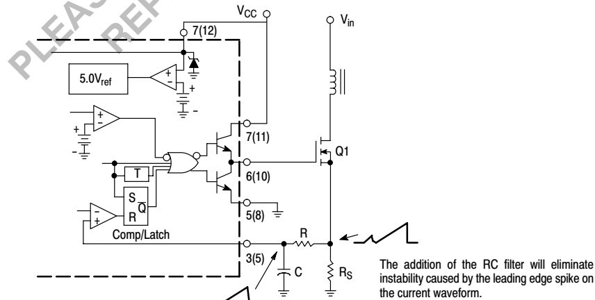
Figure 24. Current Waveform Spike Suppression
