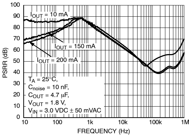
Figure 12. PSRR vs. Frequency, 1.8 V Output Voltage Option, C_{OUT} = 4.7 \mu F , C_{noise} = 10 \text{ nF}
