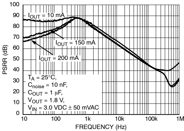
Figure 10. PSRR vs. Frequency, 1.8 V Output Voltage Option, C_{OUT} = 1 \mu F , C_{noise} = 10 \text{ nF}
