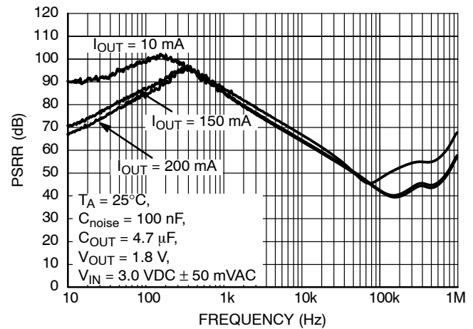
Figure 13. PSRR vs. Frequency, 1.8 V Output Voltage Option, C_{OUT} = 4.7 \mu F , C_{noise} = 100 \text{ nF}
