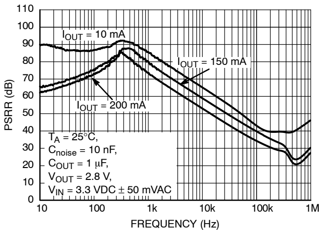
Figure 14. PSRR vs. Frequency, 2.8 V Output Voltage Option, C_{OUT} = 1 \mu F , C_{noise} = 10 \text{ nF}
