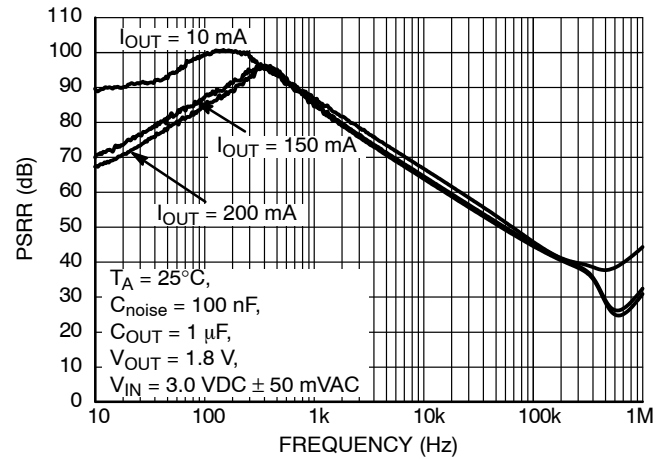
Figure 11. PSRR vs. Frequency, 1.8 V Output Voltage Option, C_{OUT} = 1 \mu F , C_{noise} = 100 \text{ nF}
