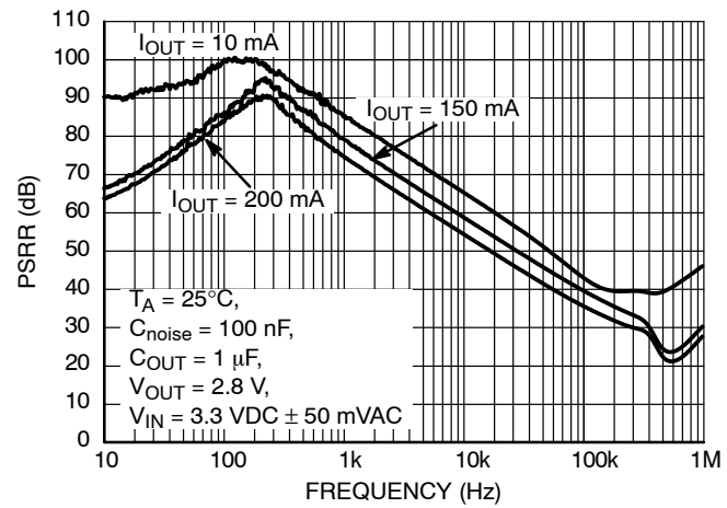
Figure 15. PSRR vs. Frequency, 2.8 V Output Voltage Option, C_{OUT} = 1 \mu F , C_{noise} = 100 \text{ nF}
