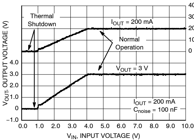
Figure 43. Thermal Shutdown Protection V_{OUT} = 3 V, C_{noise} = 100 nF, C_{OUT} = 1 \mu\text{F}
