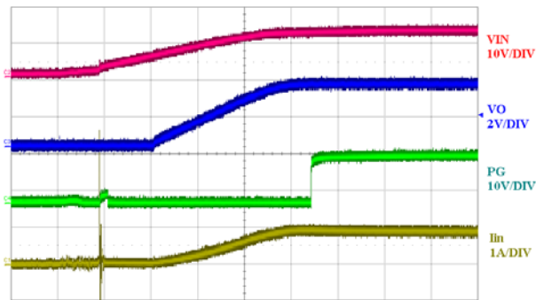
Figure 5. Start-Up into Full Load 1 \text{ms}/\text{DIV}
