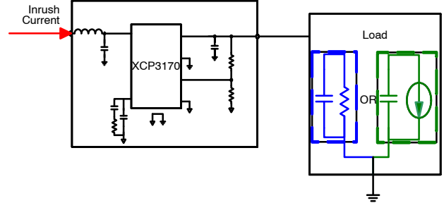
Figure 48. Load Connected to the Output Stage
