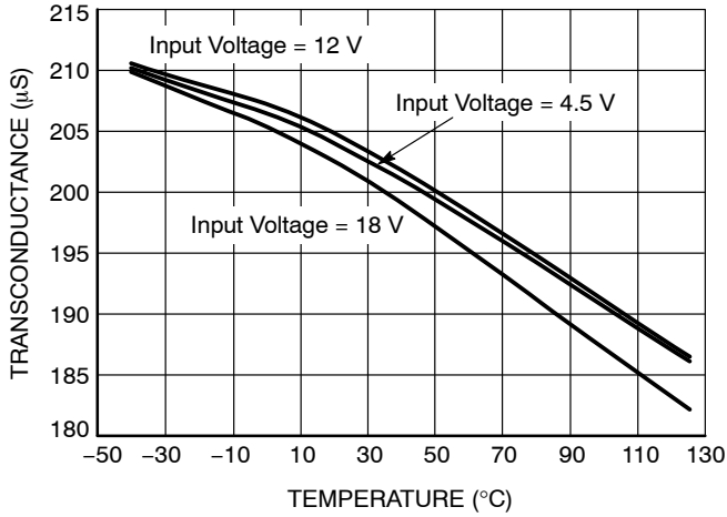
Figure 17. Transconductance vs. Temperature
