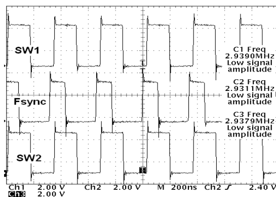
Figure 17. External Synchronization, F_{sync} = 2.93 \text{ MHz}
