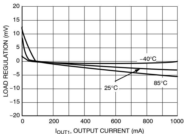
Figure 13. Load Regulation V_{IN} = 3.6\text{ V} , V_{OUT1} = 1.2\text{ V} , EN2 = \text{GND}
