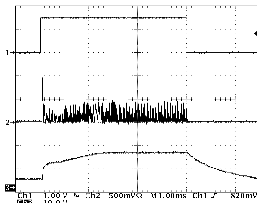
Figure 26. Operating Waveforms (Heavy Load)
