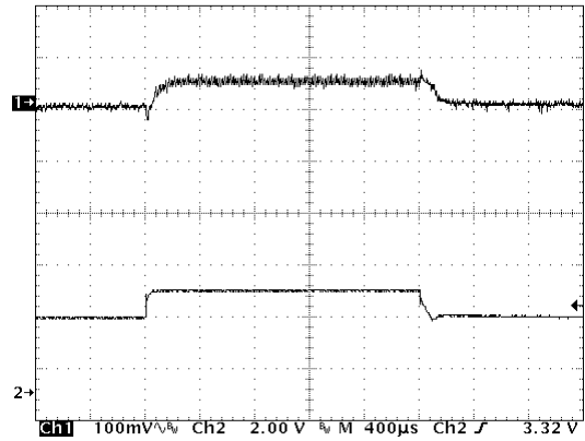
Figure 24. Line Transient Response ( V_{OUT} = 15\text{ V} )
