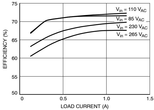
Figure 36. Converter Efficiency
