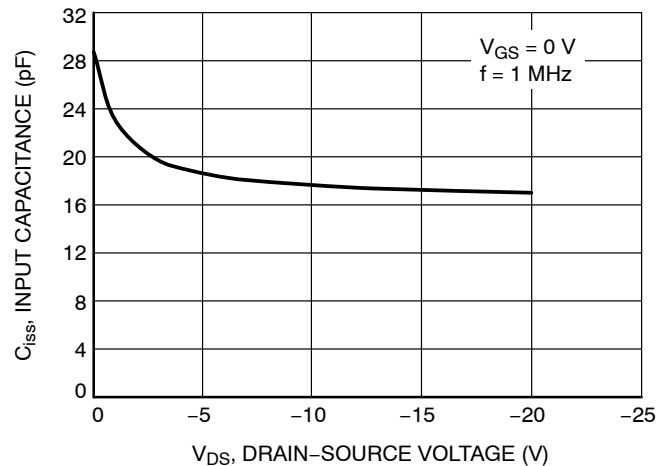
Figure 3. Input Capacitance
