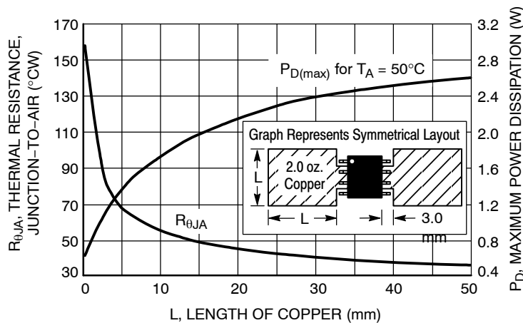
Figure 19. SOP-8 Thermal Resistance and Maximum Power Dissipation versus P.C.B. Copper Length
