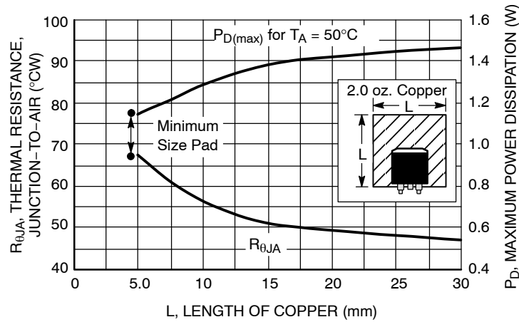
Figure 18. DPAK Thermal Resistance and Maximum Power Dissipation versus P.C.B. Copper Length
