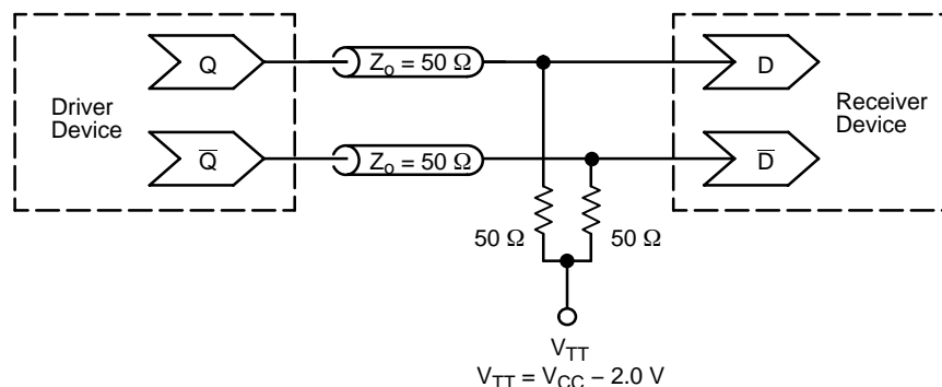
Figure 2. Typical Termination for Output Driver and Device Evaluation (See Application Note AND8020 – Termination of ECL Logic Devices.)
