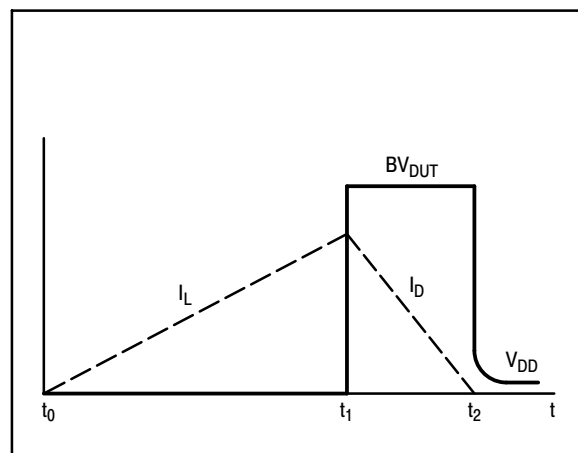
Figure 14. Current-Voltage Waveforms
