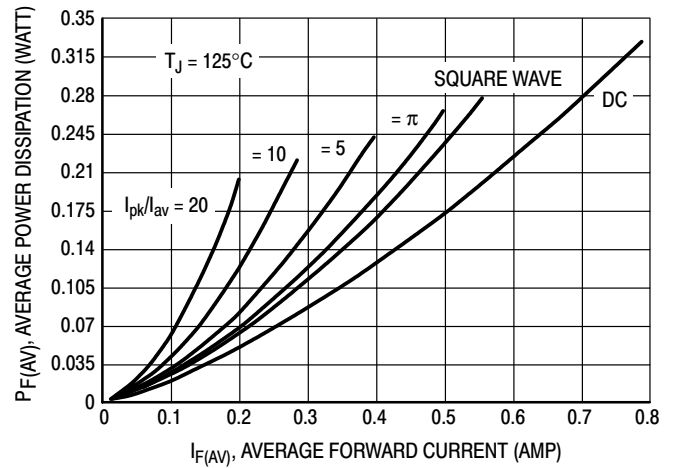
Figure 5. Power Dissipation
