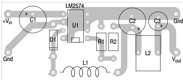
Figure 40. PC Board Layout Component Side
