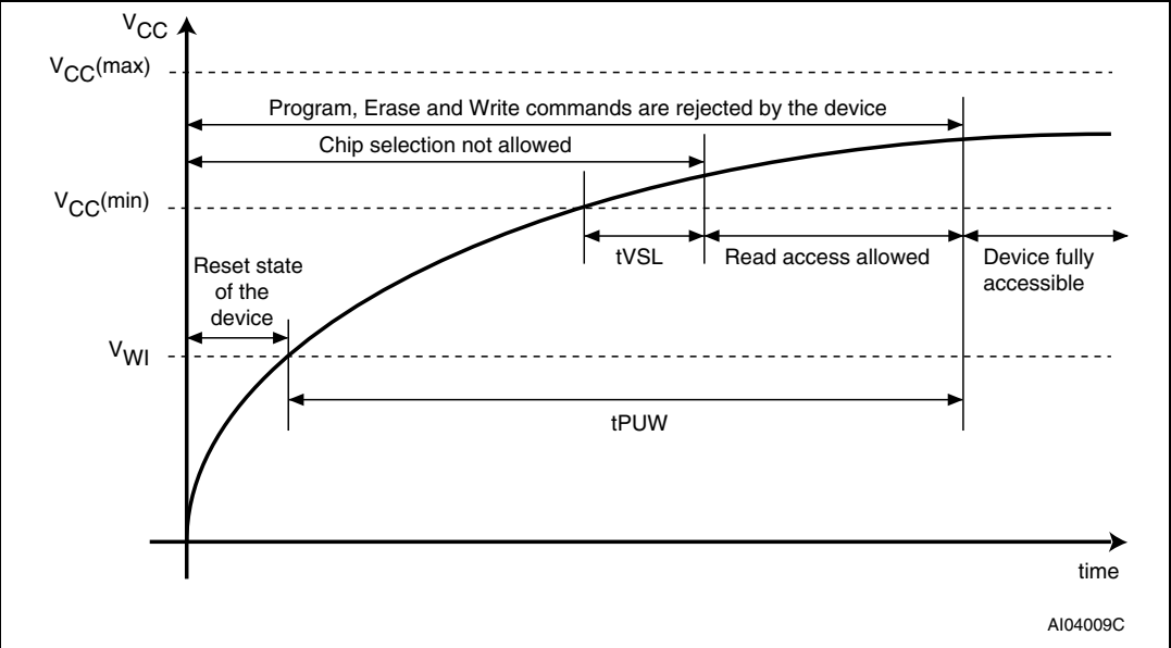
Figure 25. Power-up timing
