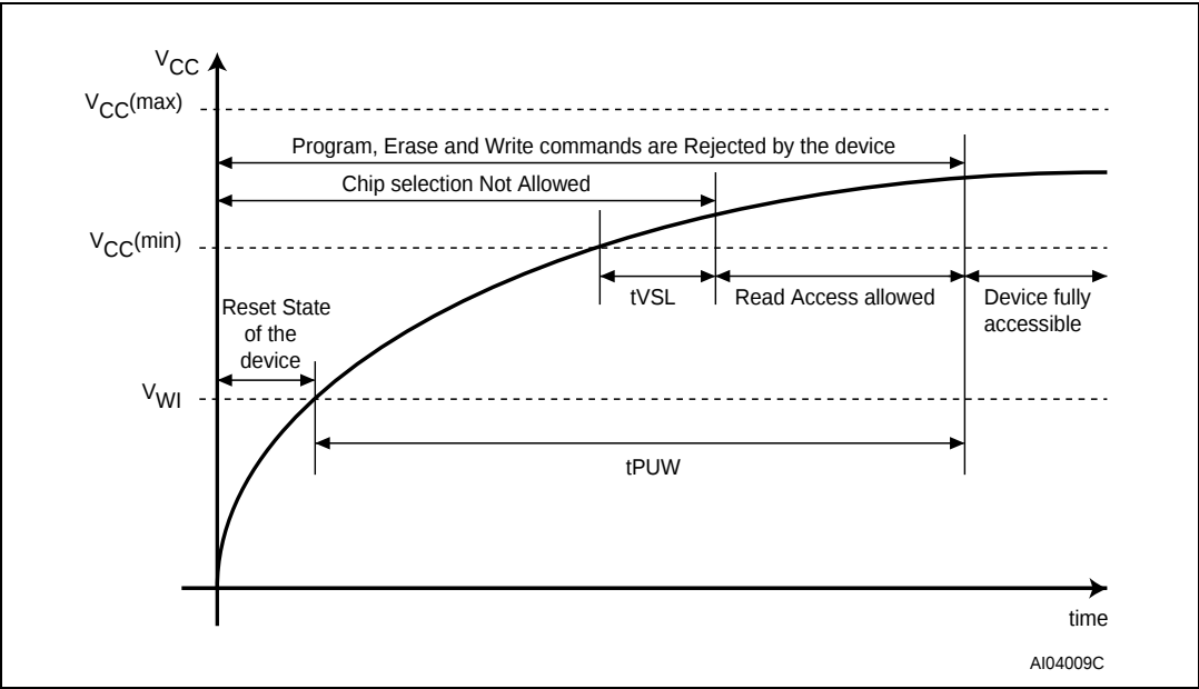
Figure 20. Power-up timing
