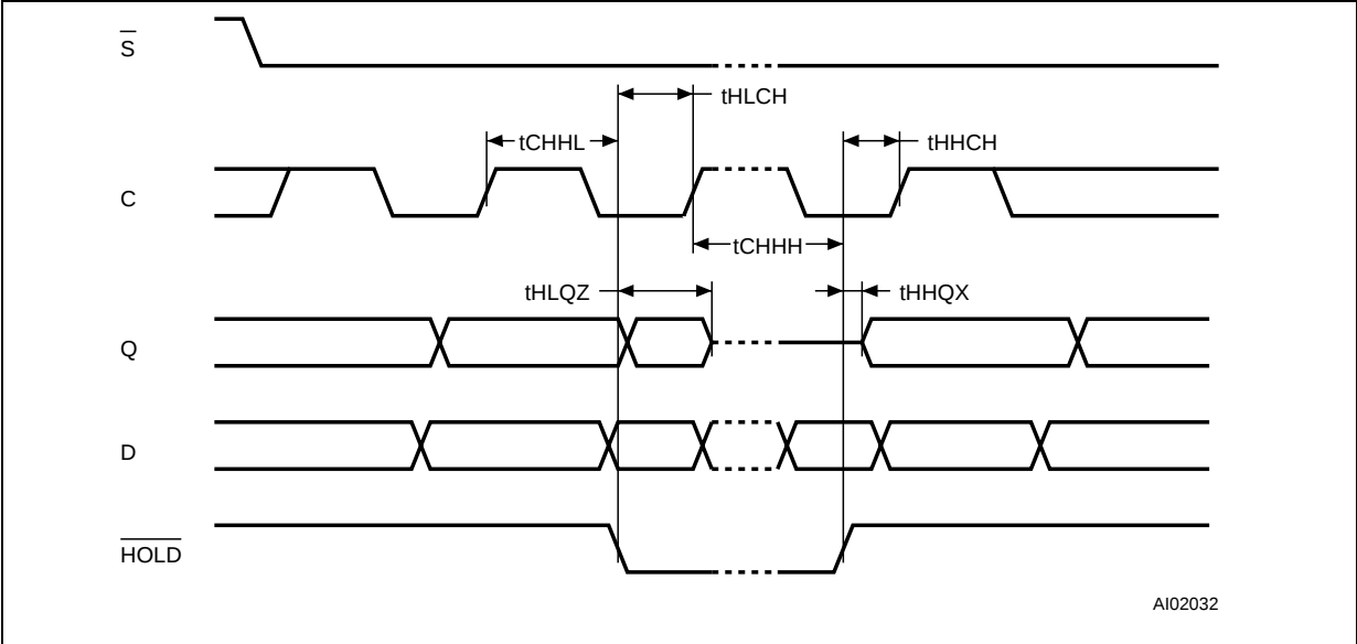
Figure 25. Hold timing
