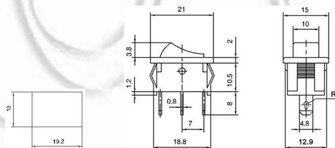
RSM102 RSM102A ON-ON RSM103 RSM103A ON-OFF-ON RSM112 RSM112A ON-(ON) SPDT 3P
