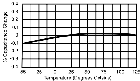
TYPICAL NPO TEMPERATURE COEFFICIENT
