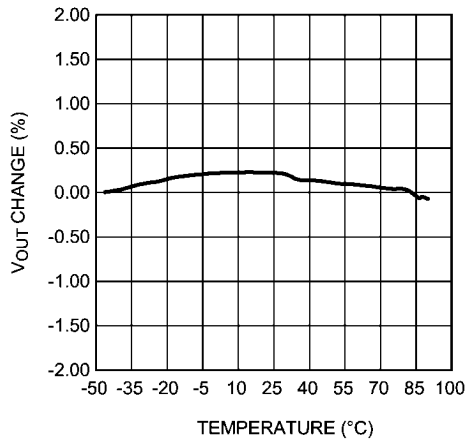
Output Voltage Change vs Temperature (LDO1) Vin = 4.3V, Vout = 3.3V, 100 mA load
