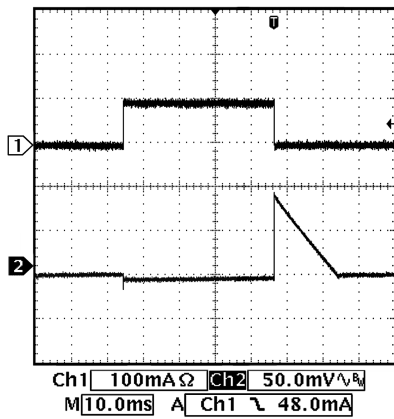
Load Transient (LDO1) 3.6 Vin, 3.3 Vout, 0 – 100 mA load
