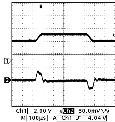
Line Transient (LDO2) 3 - 4.2 Vin, 1.8 Vout, 150 mA load
