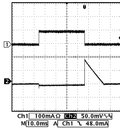
Load Transient (LDO2) 3.6 Vin, 1.8 Vout, 0 – 100 mA load
