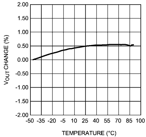
Output Voltage Change vs Temperature (LDO2) Vin = 4.3V, Vout = 1.8V, 100 mA load
