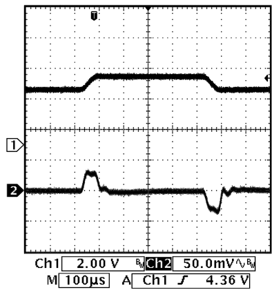
Line Transient (LDO1) 3.6 - 4.5 Vin, 3.3 Vout, 150 mA load
