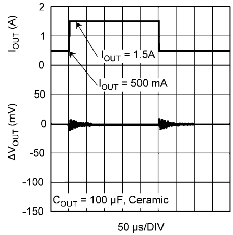
Load Transient Response, C_{OUT} = 100 \mu\text{F} Ceramic
