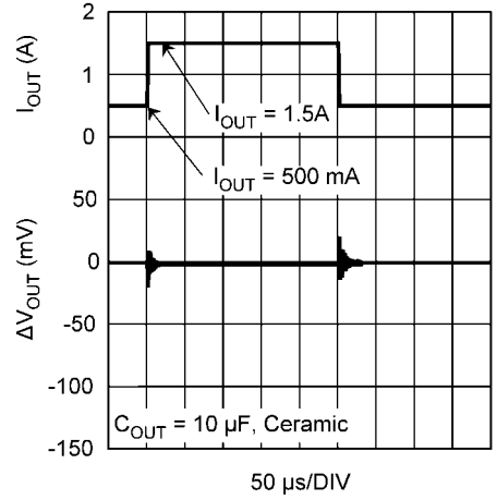
Load Transient Response, C_{OUT} = 10 \mu\text{F} Ceramic
