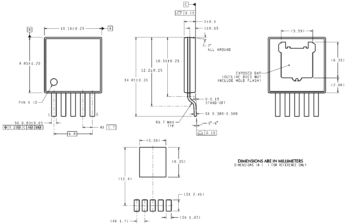
TO-263 THIN, 5 Lead, Molded, 1.7mm Pitch, Surface Mount NS Package Number TJ5A
