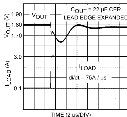
FIGURE 7. 22 µF Ceramic Output Capacitor
