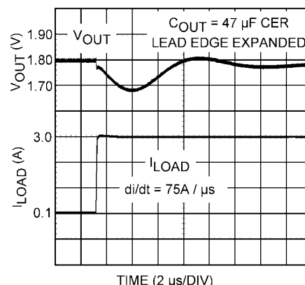
FIGURE 8. 47 µF Ceramic Output Capacitor
