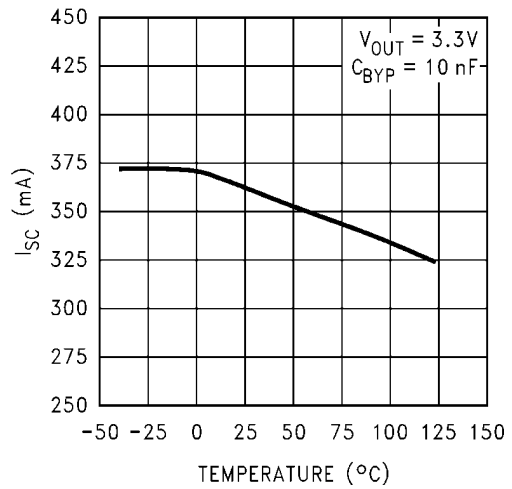
Instantaneous Short Circuit Current
