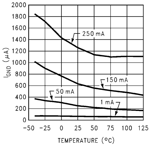
I GND vs Load and Temperature
