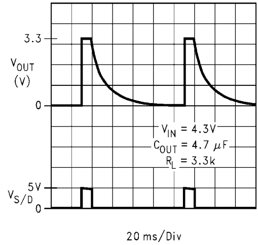
Turn-Off Waveform
