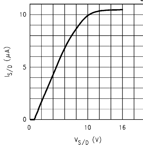
Shutdown Pin Current vs Shutdown Pin Voltage
