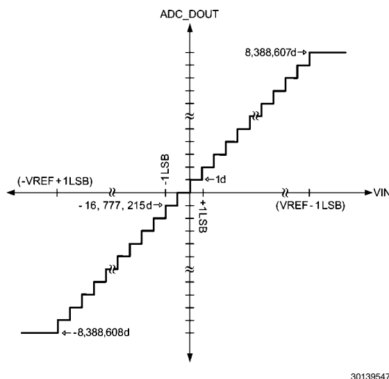
FIGURE 31. ADC_DOUT vs. V_{IN} of a 24-Bit Resolution ( V_{REF} = 5.5V , Gain = 1).
