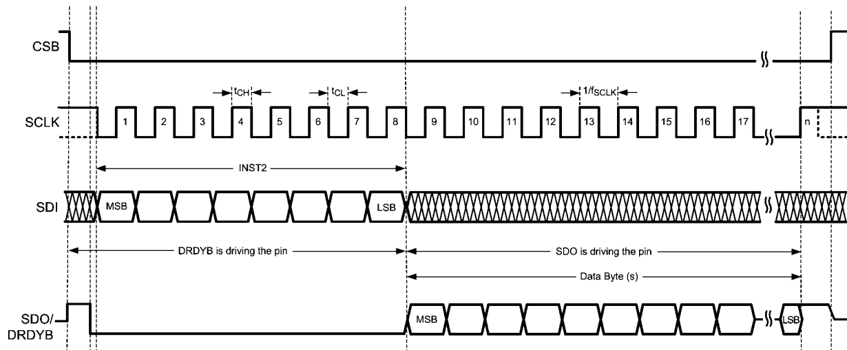
FIGURE 2. Timing Diagram
