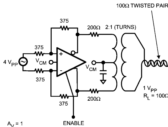
FIGURE 10. Transformer Out Low Impedance Load
