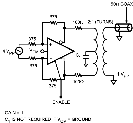
FIGURE 11. Driving 50Ω Test Equipment
