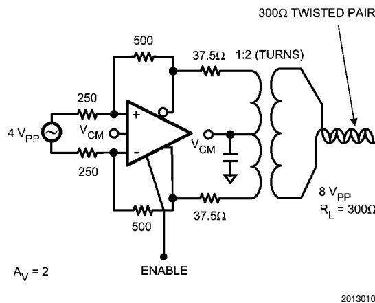
FIGURE 8. Transformer Out High Impedance Load
