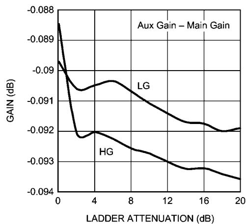
Gain Matching vs. Ladder Attenuation
