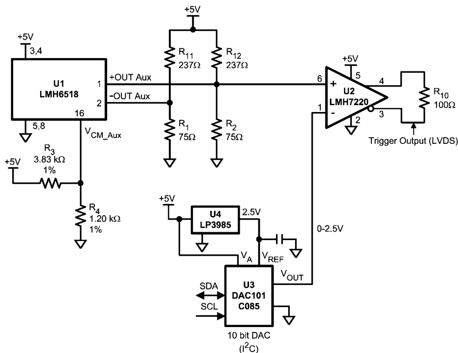
FIGURE 12. Single-Ended Trigger from LMH6518 Auxiliary Output
