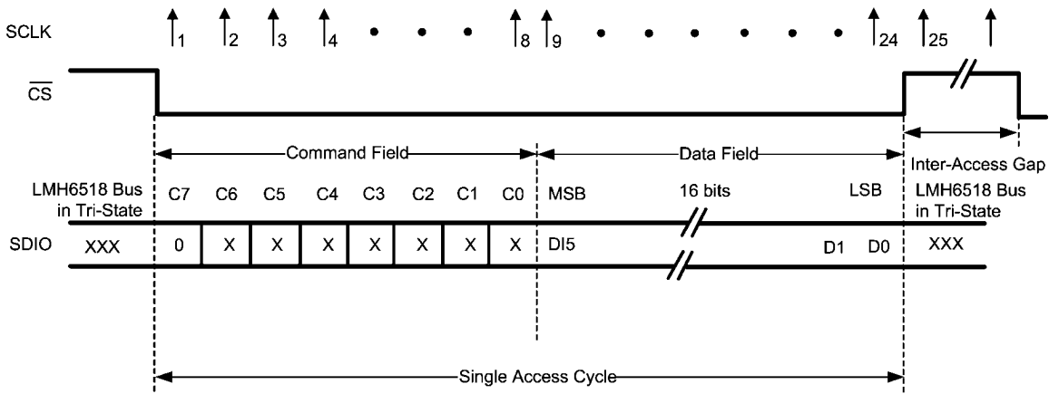
FIGURE 9. Serial Interface Protocol- Write Operation
