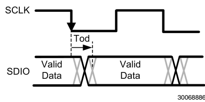
FIGURE 10. Read Timing
