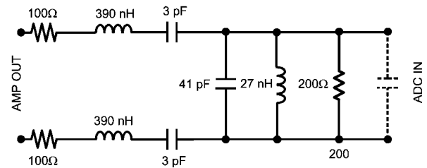
FIGURE 18. Bandpass Filter Center Frequency is 140 MHz with a 20 MHz Bandwidth Designed for 200Ω Impedance
