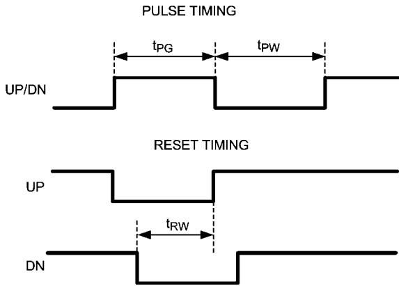
FIGURE 17. Pulse Mode Timing
