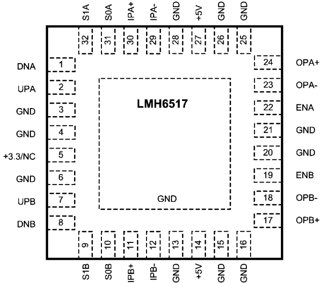
FIGURE 16. Pin Functions for Pulse Mode
