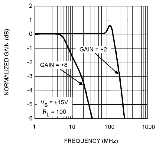
Frequency Response
