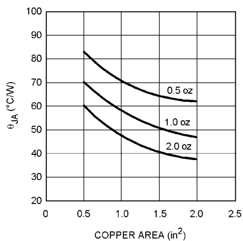
Thermal Performance of 8ld-PSOP
