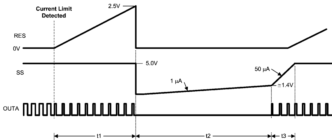
FIGURE 7. Hiccup Over-Load Restart Timing
