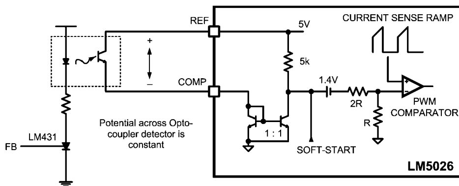
FIGURE 4. Opto-Coupler to LM5026 COMP Interface
