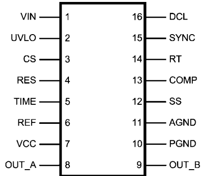
16-Lead TSSOP
