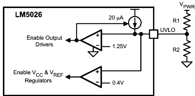
FIGURE 13. Basic UVLO Configuration
