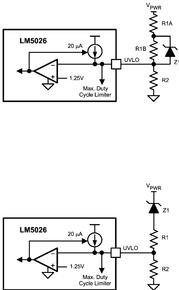
FIGURE 17. Altering the Slope of Duty Cycle vs. V_{PWR}
