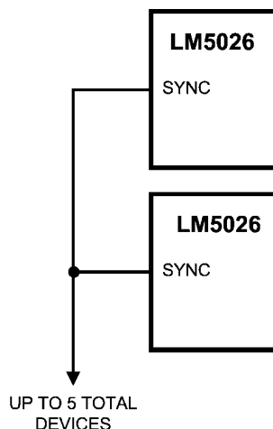
FIGURE 9. Sync from Multiple Devices
