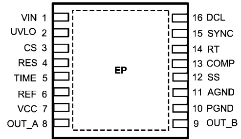
16-Lead LLP
