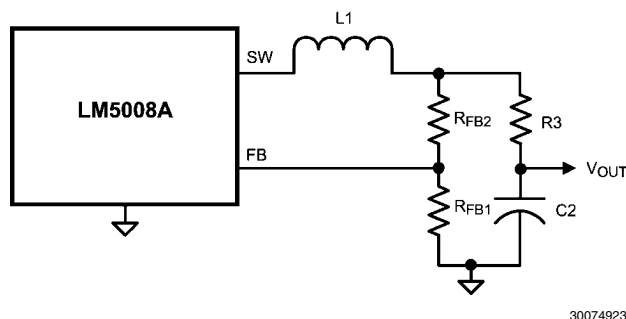
FIGURE 9. Alternate Minimum Output Ripple
