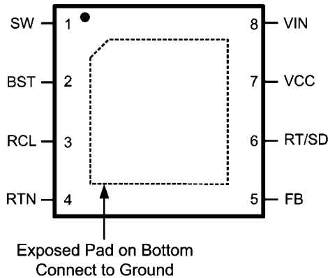
Top View 8-Lead LLP
